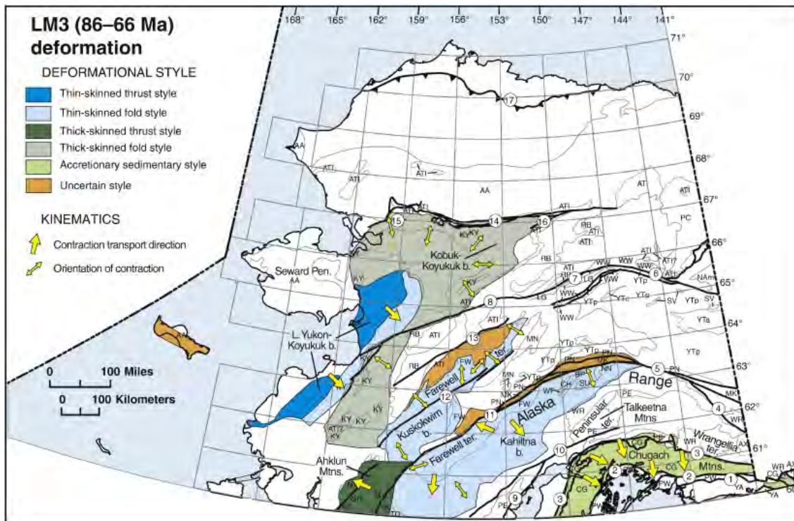
Figure 7-5: West-Central Alaska Deformation 86–66 Ma
