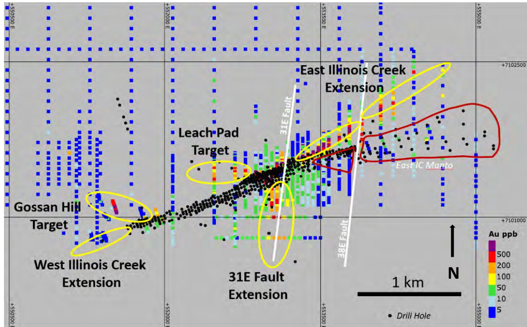
Figure 9-6: Gold Soil Geochemistry and Exploration Targets Near the Illinois Creek Deposit
