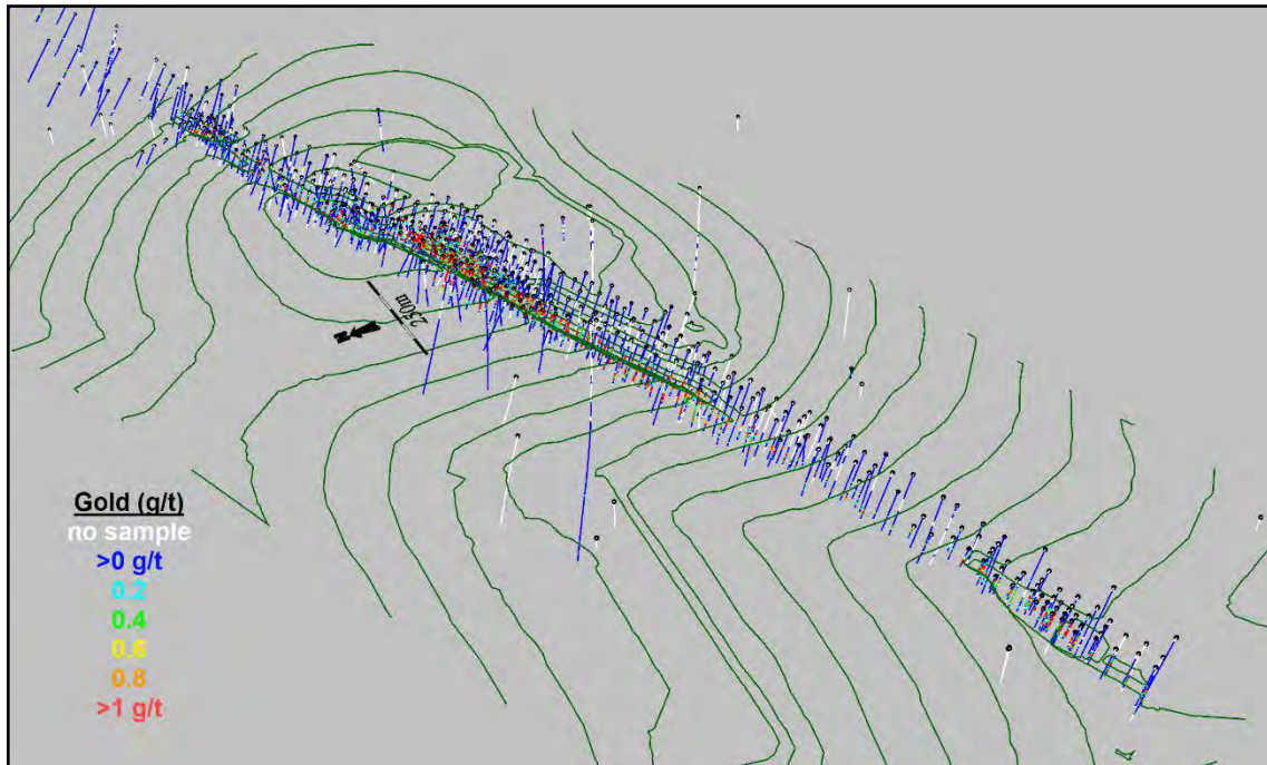
Figure 14-5: Isometric View of Gold Data in Drilling following Treatment of Unsourced Intervals
