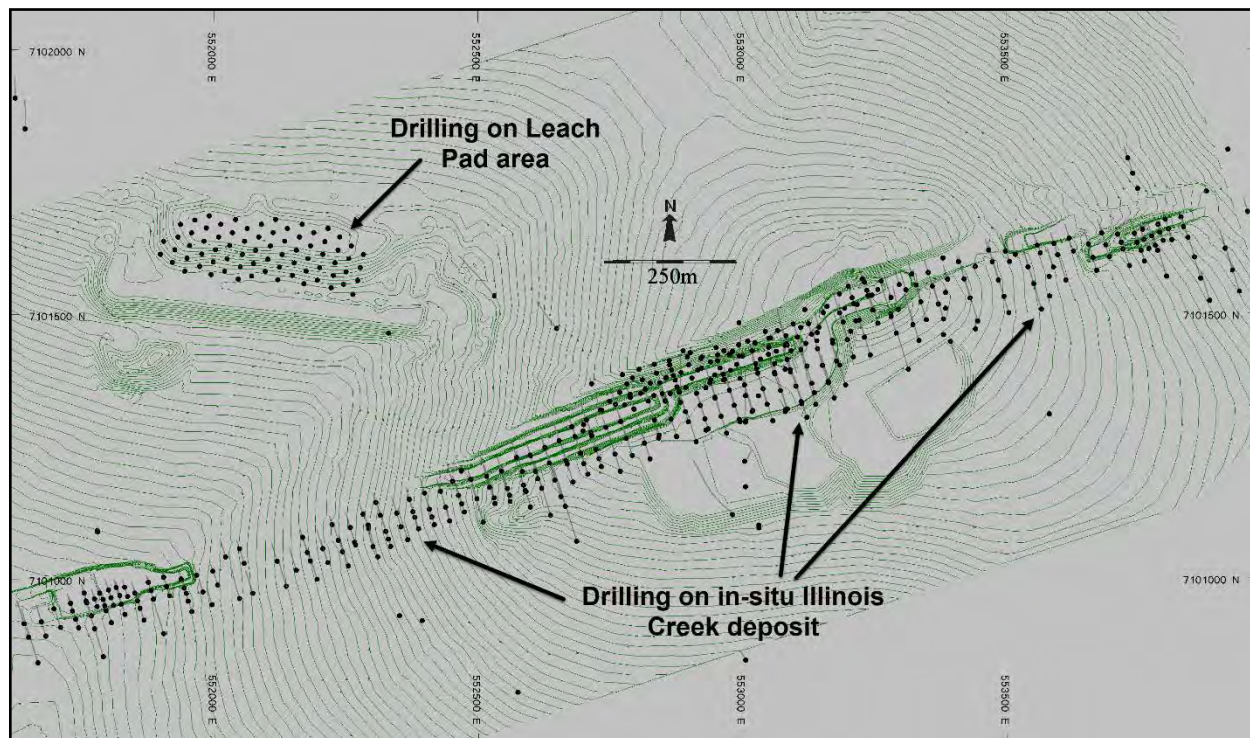
Figure 14-17: Plan View Showing Drilling on the Illinois Creek Deposit and in the Leach Pad Area
