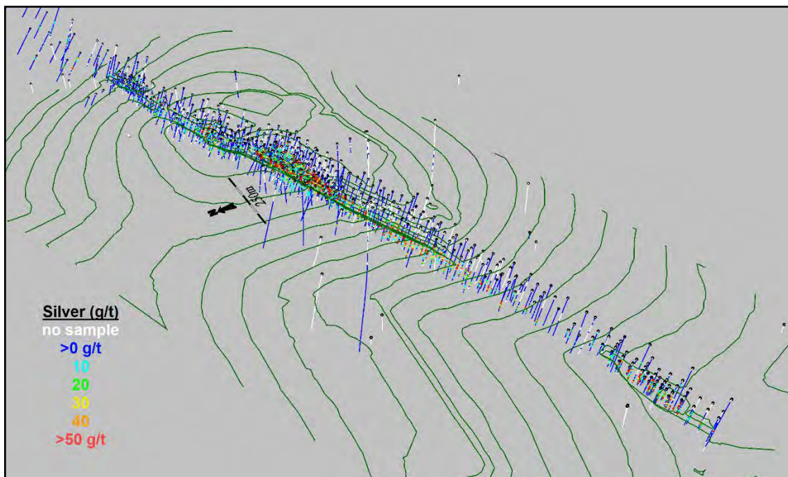
Figure 14-6: Isometric View of Silver Data in Drilling following Treatment of Unsourced Intervals
