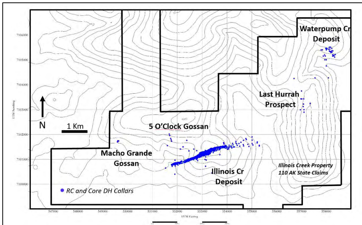
Figure 6-1: Plan Showing Mineralized Zones and Drill Hole Locations
