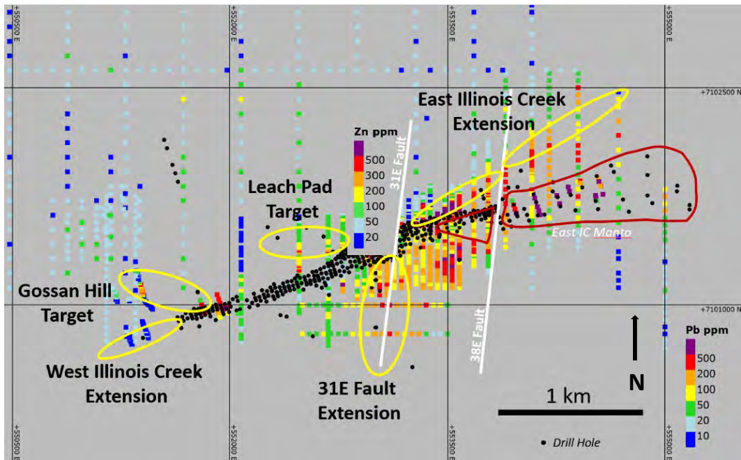
Figure 9-10: Lead Soil Geochemistry and Exploration Targets Near the Illinois Creek Deposit
