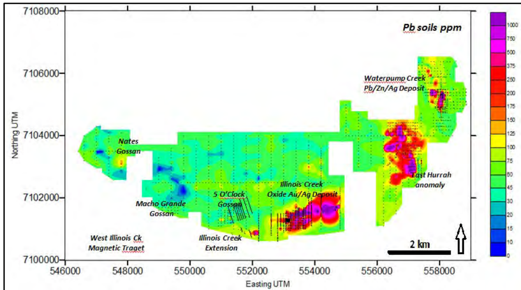
Figure 9-3: Lead Soil Geochemistry – Illinois Creek Property
