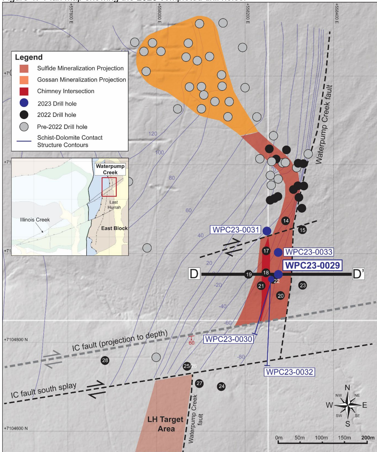
Figure 1. Plan map showing the 2023 completed drill holes.
